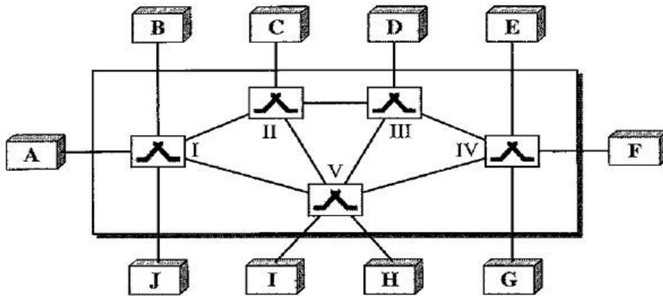
Figure 4 Switched Network
